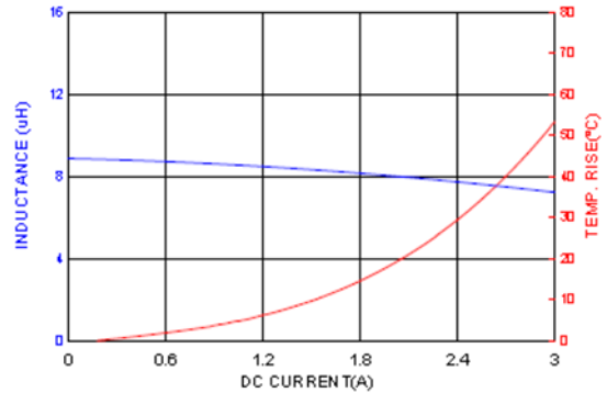
HMPL0512HP-220
